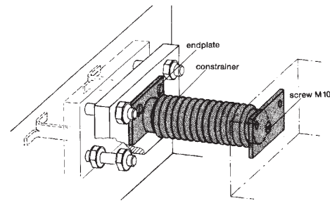
Mounting example
