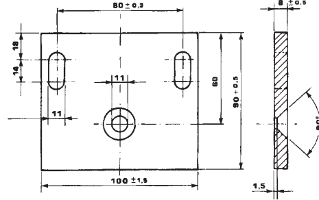
Dimensions, endplate in mm
