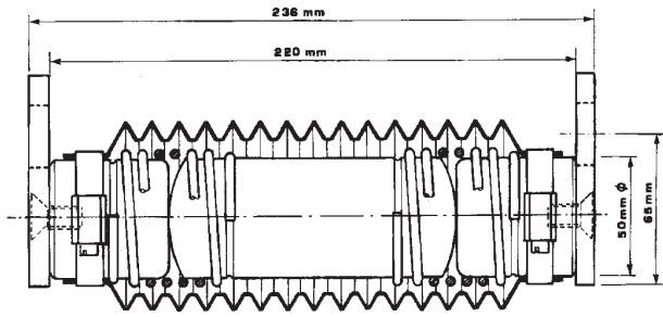
Dimensions, Horizontal Constrainer incl. endplates
